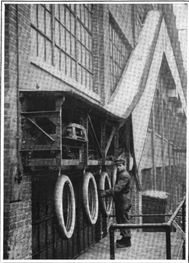
Fig. 30—Where there is considerable congestion in a shop, it may be desirable to hang conveyor systems and similar equipment on the outside of buildings. A case in point is seen in the accompanying illustration, which shows a view of a conveyor system installed in the Studebaker Corporation factory for handling tires, wheels and hubs. The conveyor is an endless chain with hooks for carrying the work.
